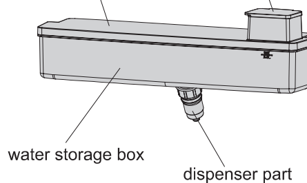
water storage box cover
